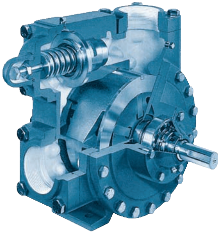
LGLD4 cutaway
