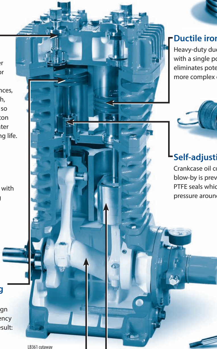
LB361 cutaway
