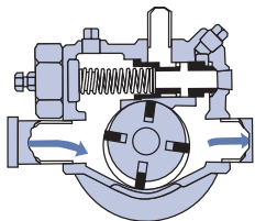
FIGURE 3. Combination relief/bypass valve
